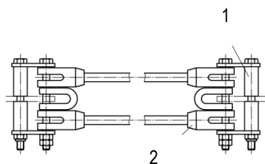
Fig. 2: Damping device
