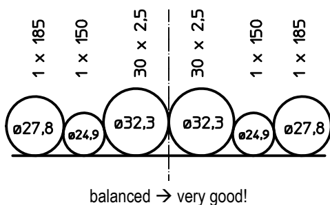
Fig 40: Cable balance
