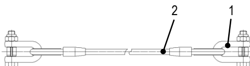
Fig 22: Stress-relieving cable
