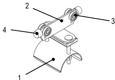
Fig 49.: Cable trolley
