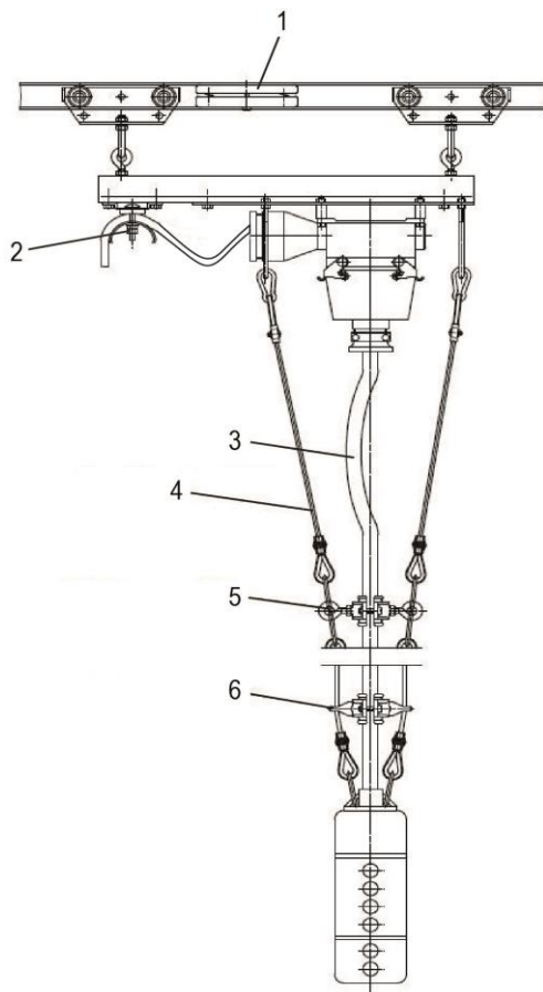
Fig. 6: Ideal control trolley
