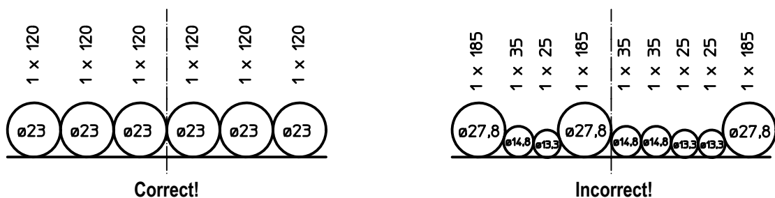
Fig. 38.: Diameter differences
