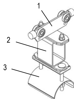
Fig. 16: Towing trolley
