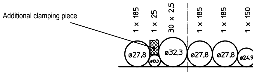
Fig. 39: Using clamping pieces
