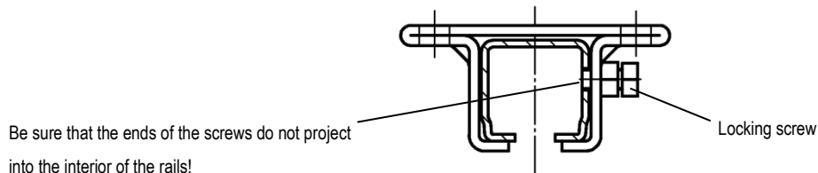
Fig. 3: Securing rails against slipping out
